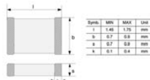
H=0.9mm, W=1.75mm, D=0.9mm
